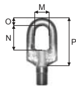
Swivel eye
